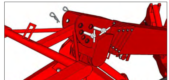
(Fig. 2): Place and orient the AWP so that it is directly in front of the SPYDERCRANE with the end of the yoke pointing at the Boom Tip.
