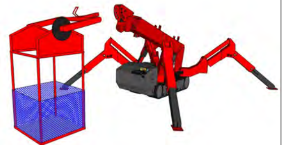
(Fig. 1): Place and orient the AWP so that it is directly in front of the SPYDERCRANE with the end of the yoke pointing at the Boom Tip.
